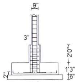
Section X-X
