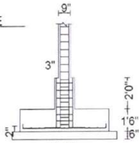
Section X-X
